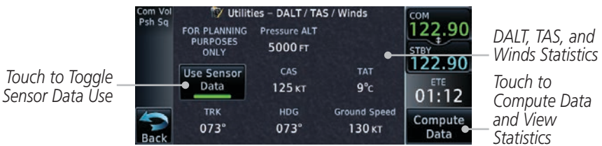
Figure 14-37 Utility DALT/TAS/Winds Page Using Sensor Data and Pressure Altitude
