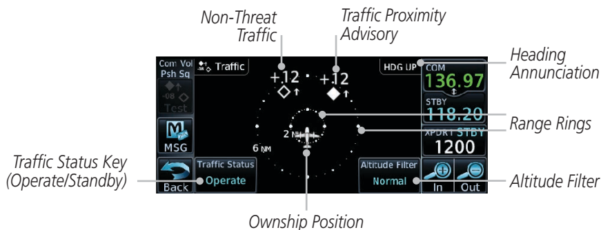
Figure 9-8 Traffic Page
