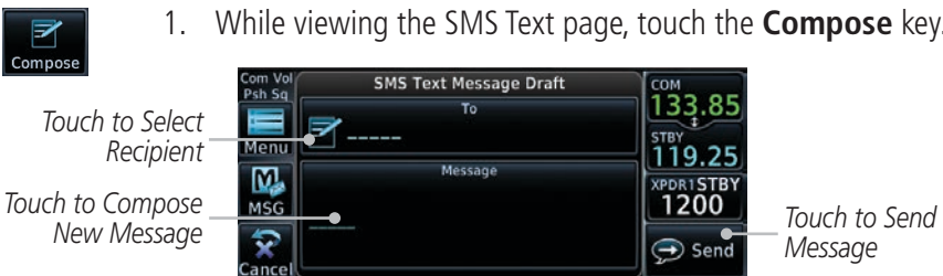
Figure 13-23 Compose a New SMS Text Message
