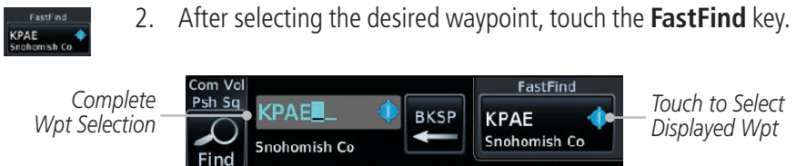
Figure 1-28 Select Characters for FastFind to Predict a Waypoint - KPAE Selected
