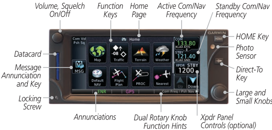
Figure 1-2 GTN 650 Front Panel
