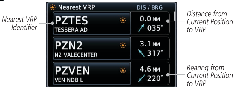
Figure 12-11 Nearest VRPs
