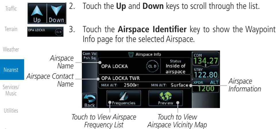
Figure 12-19 Nearest Airspace Waypoint Information
