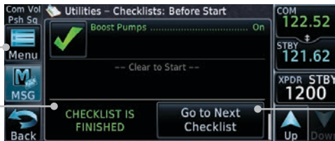
Figure 14-54 Checklist Completion
