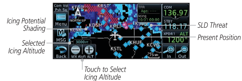
Figure 11-42 Icing
