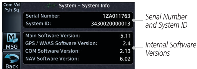
Figure 15-5 System Status Version Information
