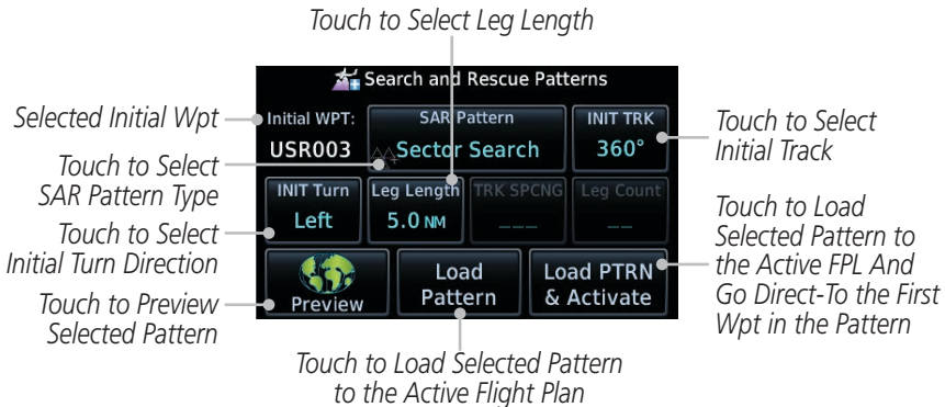
Figure 4-37 Search and Rescue Sector Search Pattern Page
