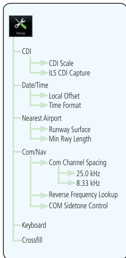
Figure 15-19 System Setup Functions
