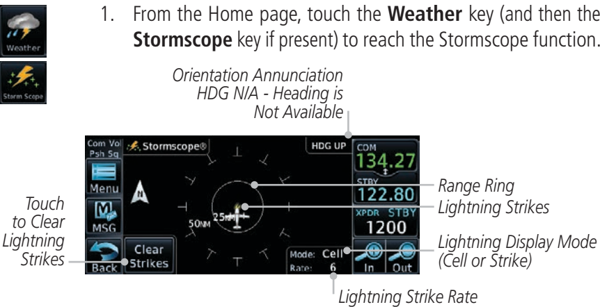
Figure 11-49 Stormscope Display (360° Display View Shown)
