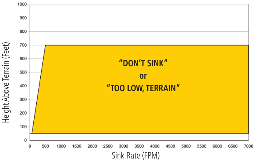
Figure 10-50 Negative Climb Rate (NCR) Sink Rate
