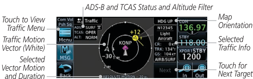
Figure 9-13 Absolute Motion (White Vectors)
