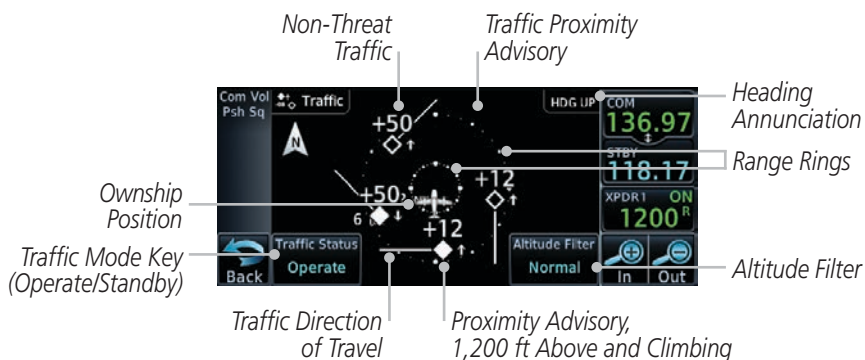
Figure 9-5 Traffic Page
